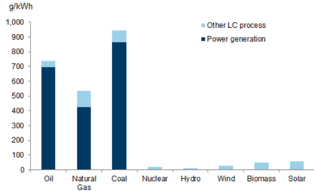
Exhibit 13: Environmental load of EVs varies widely depending on power mix
