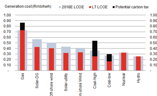
Exhibit 27: Power generation cost - now and potential outlook The addition of carbon tax or cost of carbon capture will swing the economics
